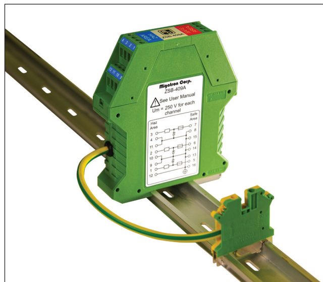
ZSB-409A and Grounding Block
